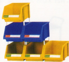
A020 STORAGE BINS 疊式零件箱 A. W120 X D180 X H80 mm 60pcs/ctn B. W150 X D250 X H120 mm 36pcs/ctn C. W200 X D350 X H150 mm 18pcs/ctn D. W200 X D450 X H177 mm 12pcs/ctn E. W300 X D450 X H177 mm 12pcs/ctn
