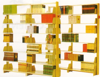
CD-19 圖書架 BOOK SHELVES A. SINGLE SIDE W965 X D305 X H2448 mm B. DOUBLE SIDE W965 X D480 X H2448 mm C. ADDITIONAL W900 mm
